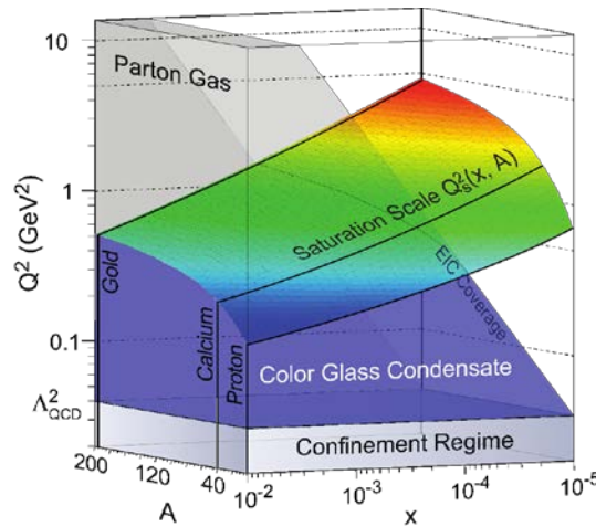
Figure 2: The conjectured QCD landscape showing the resolving power of the probe (increasing upward) vs. energy (increasing toward the right), as a function of the atomic number of the nucleus being probed.
