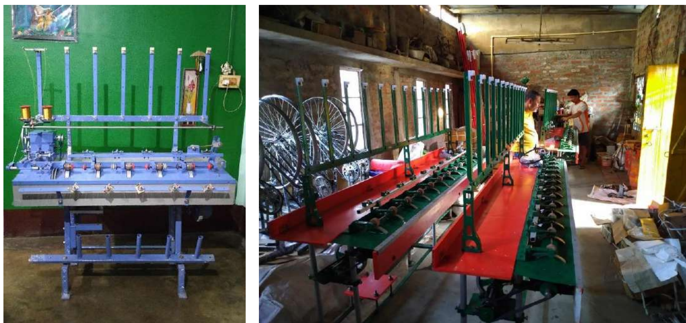
Figure 27: Hank to Bobbin yarn winding machine
