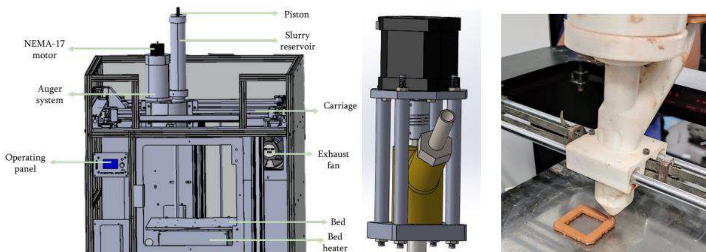
Figure 51: Bacteria-Mediated 3-D Printing of Green Bricks
