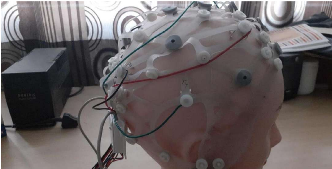
Figure 48: EEG Device with dry electrodes for diagnosis of Epilepsy
