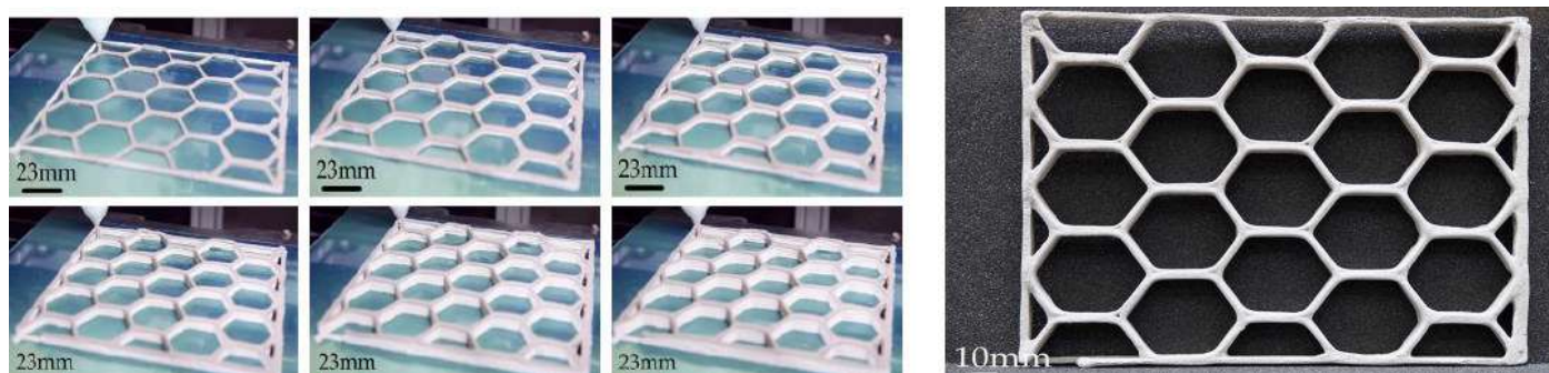
Figure 50: Honeycomb mechanical structure, 3-D printing using bacteria
